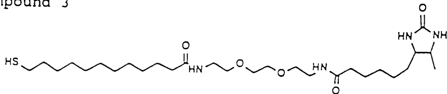
desthio compound 3
